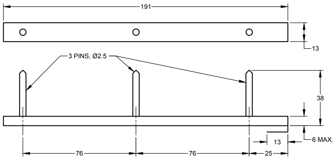
FIG. 2 CRITICAL DIMENSIONS OF SPECIMEN SUPPORT
