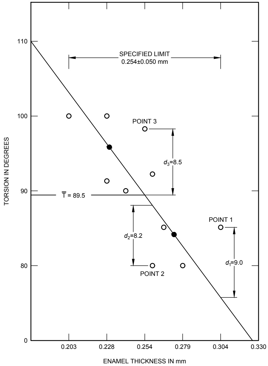
FIG. 3 PLOT OF TORSION DATA SHOWN IN TABLE 1
