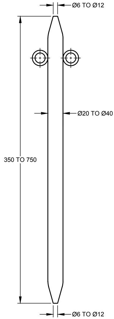
FIG. 2 OPEN TYPE SAMPLING TUBE FOR HOMOGENEOUS LIQUIDS
