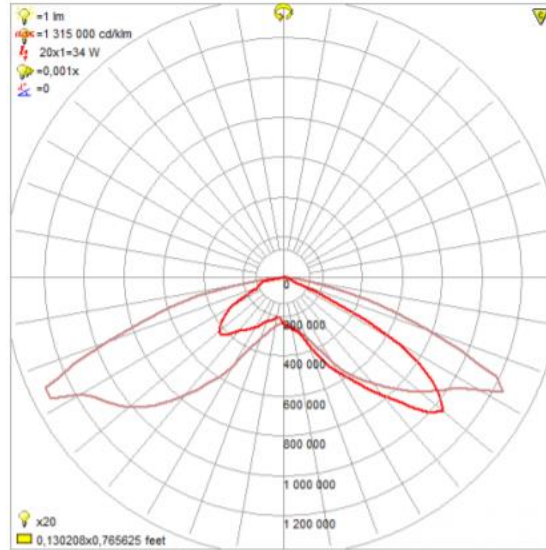
Fig. 5 Polar Diagram
