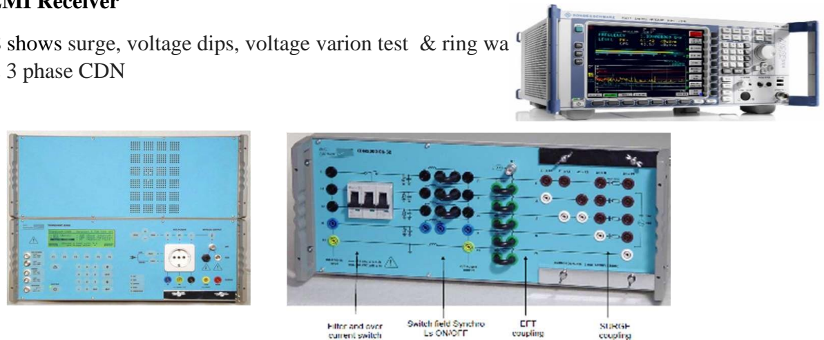
Fig. 18 Surge, Voltage Dips, Voltage Variation Test & Ring Wave Test - Generator, 1 Phase CDN & 3 Phase CDN
