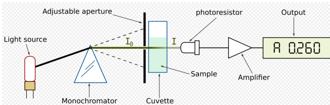
Fig. 9 Block Diagram of Spectrometer
