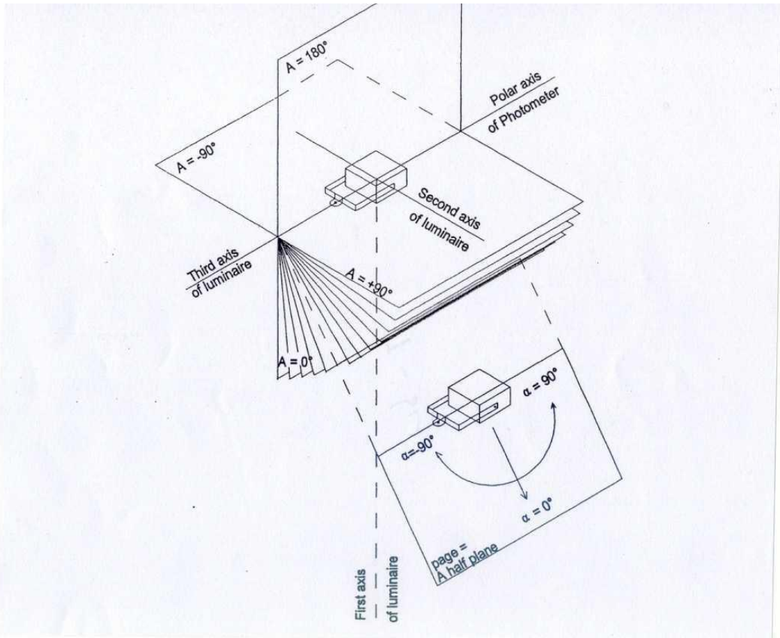
Fig.2 Luminaire Orientation for A, Alpha Goniometry
