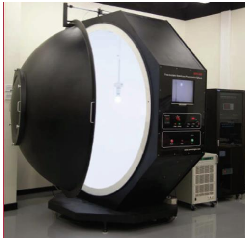
Fig.7 Integrating Sphere
