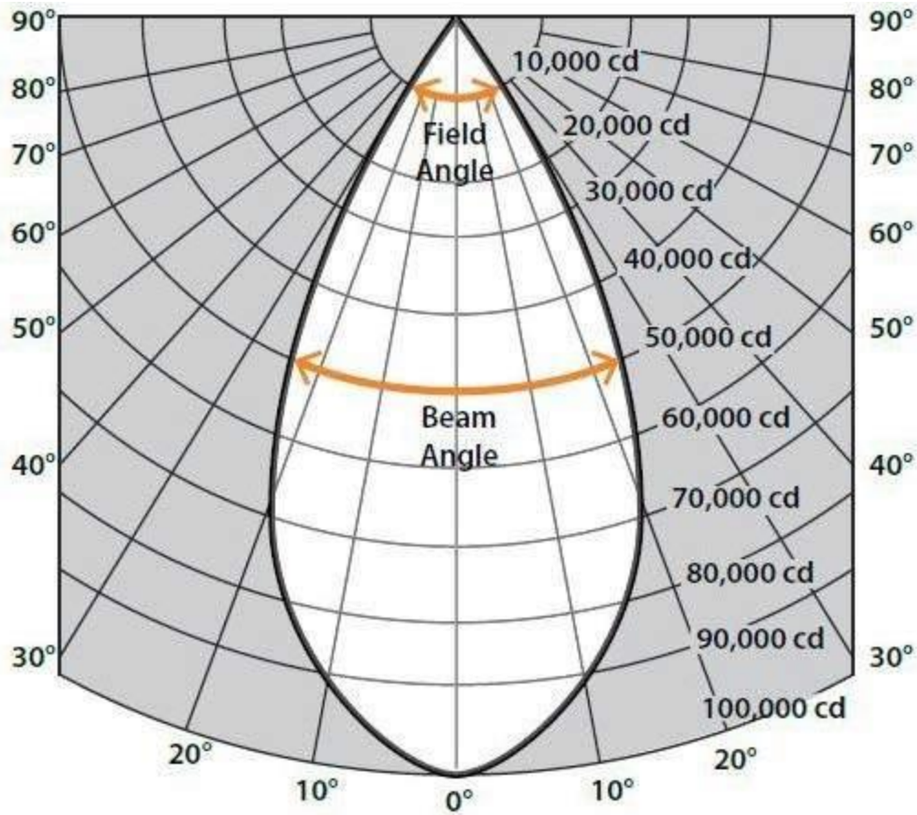
Fig. 22 NEMA Classification
