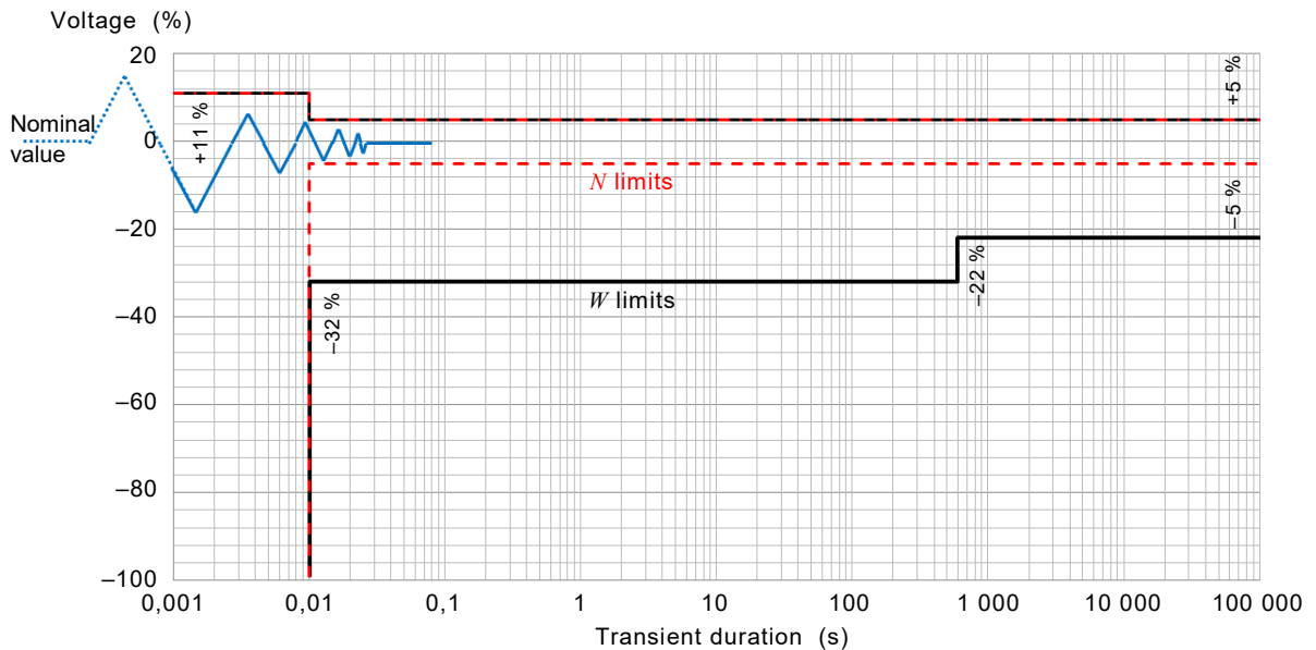
Figure E.1 – Example: Narrowband validation of dynamic voltage response
