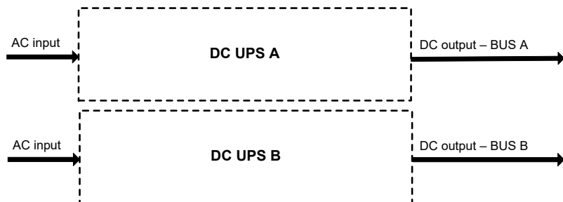
Figure A.5 – Dual bus DC UPS
