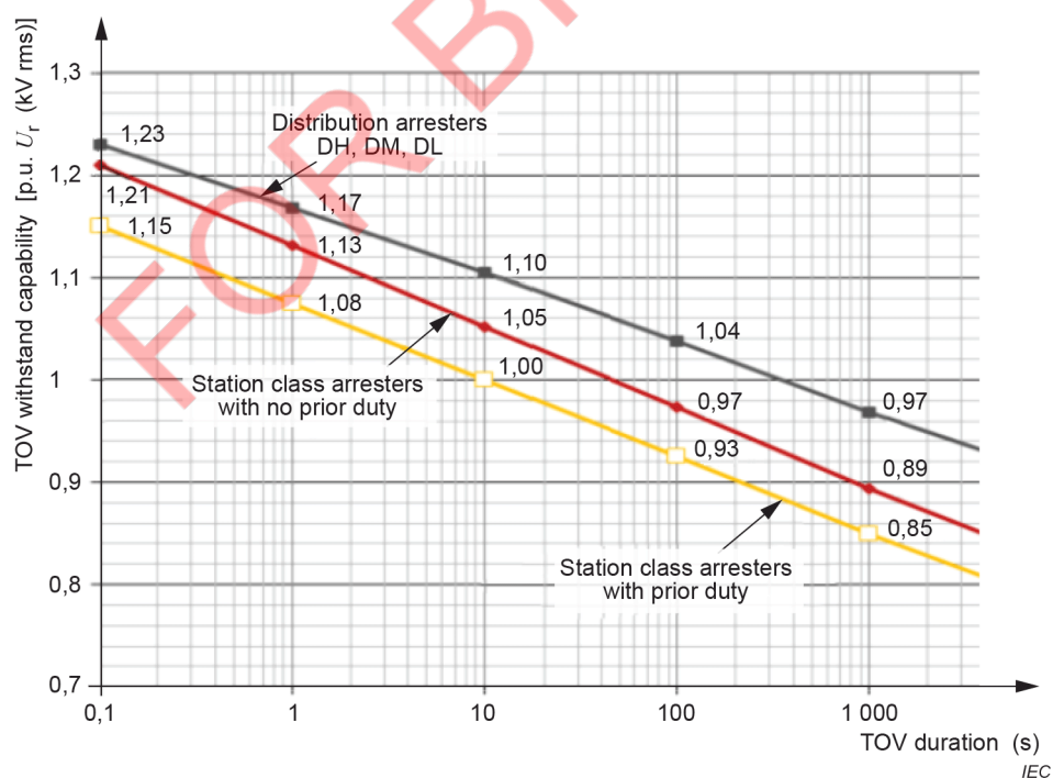
Figure 6 – Examples of TOV curves
