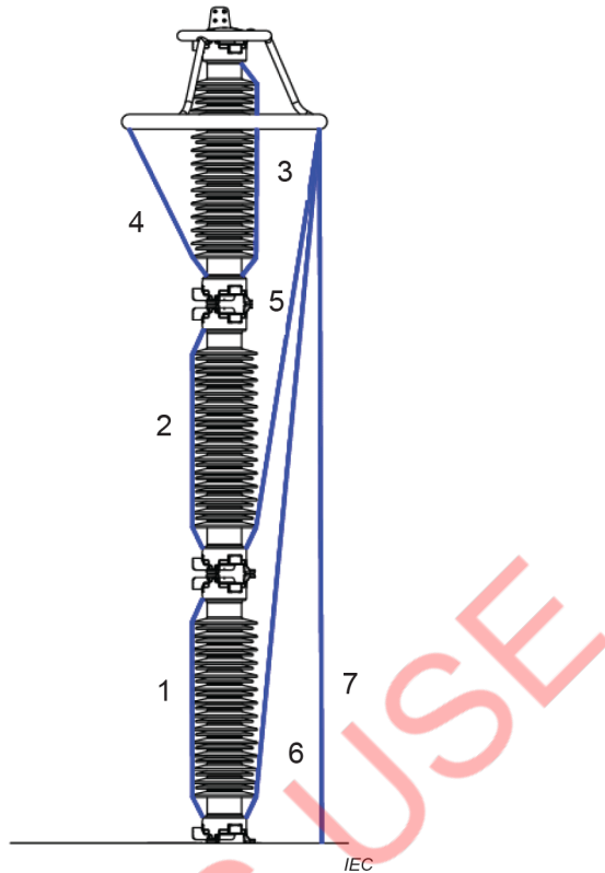
Figure 1 – Possible arcing distances (7 paths to consider for this example) for a multi-unit arrester (from CIGRÉ 696-2017)
