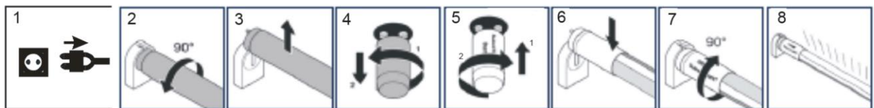
Fig. 9 Schematic Steps of Removing a Fluorescent Lamp and Inserting a Double-Capped LED Lamp Designed to Retrofit Linear Fluorescent Lamp
