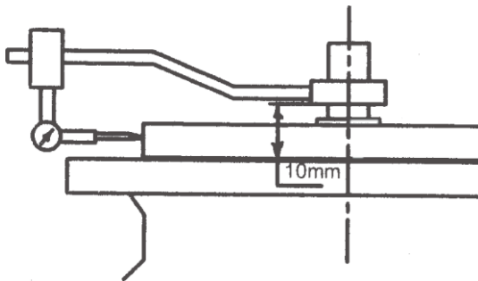
FIG. 9 MEASUREMENT OF CONCENTRICITY OF MOUNTING SPIGOT AND SHAFT
