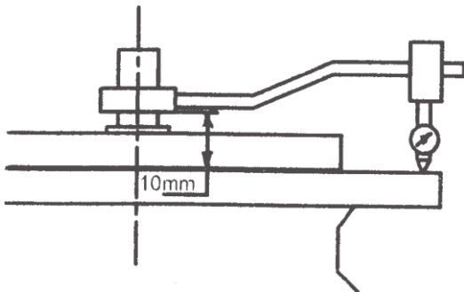
FIG. 10 MEASUREMENT OF FACE RUNOUT
