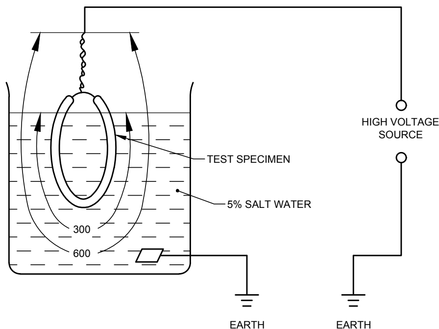
FIG. 1 IMMERSION TEST PLAN
