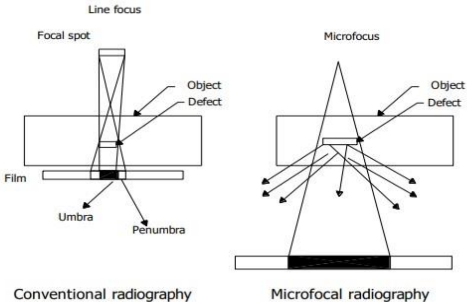
FIG. 2 MICROFOCAL SPOT MAKES IT POSSIBLE TO HAVE PROJECTIVE MAGNIFICATION AND HIGH CONTRAST RADIOGRAPHS DUE TO DECREASED SCATTER RADIATION
