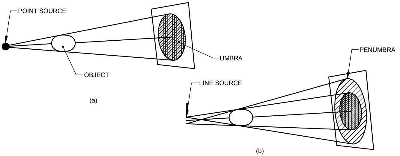
FIG. 1 IMAGE DUE TO POINT SOURCE OF RADIATION AND LINE SOURCE OF RADIATION
