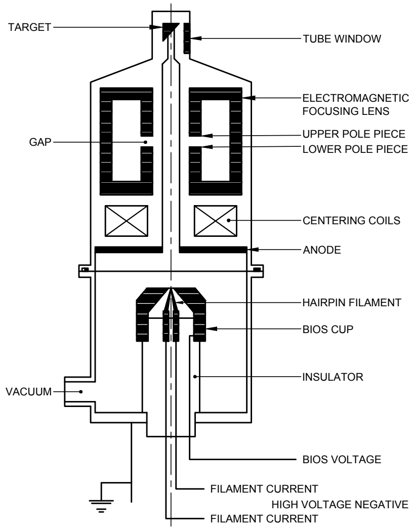
FIG. 3 TYPICAL COMPONENT IN MICRO-FOCUS X-RAY UNIT
