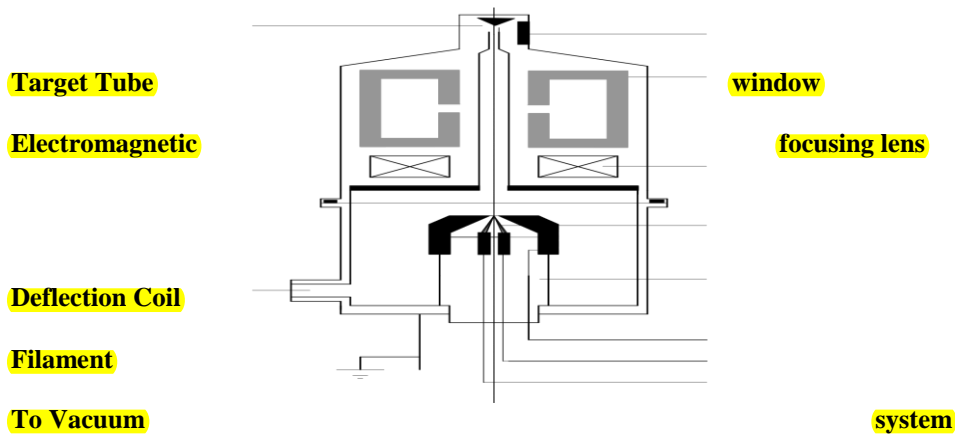
FIG. 3 TYPICAL COMPONENTS IN MICRO-FOCUS X-RAY UNIT
