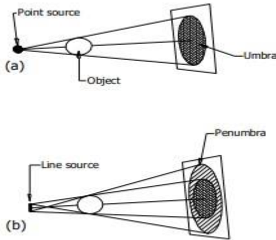
FIG. 1 IMAGE DUE TO POINT SOURCE OF RADIATION AND LINE SOURCE OF RADIATION
