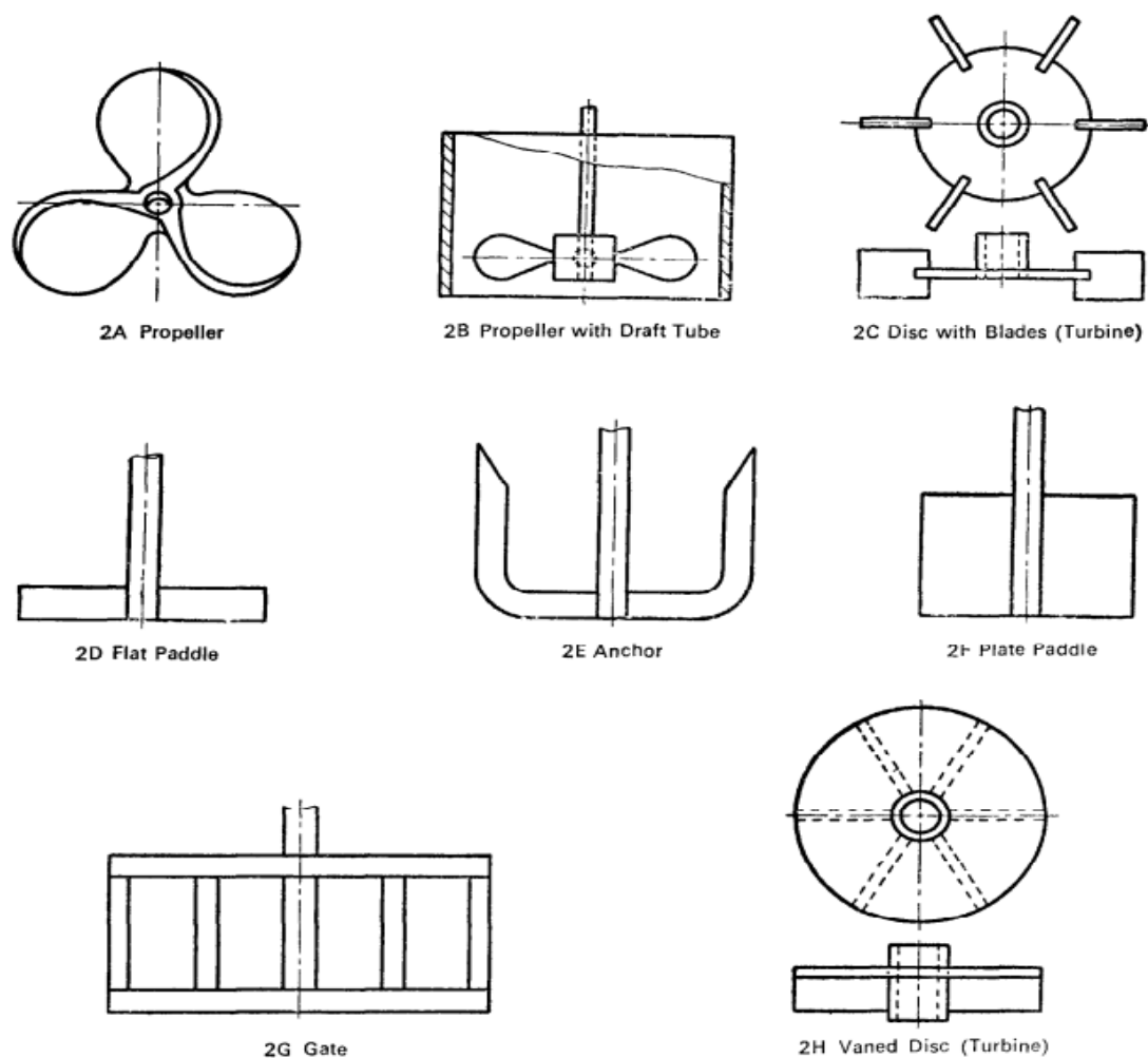
FIG. 2 TYPES OF IMPELLERS
