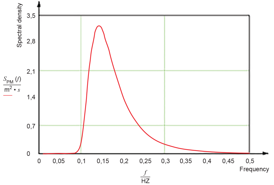
Figure C.1 – PM spectrum
