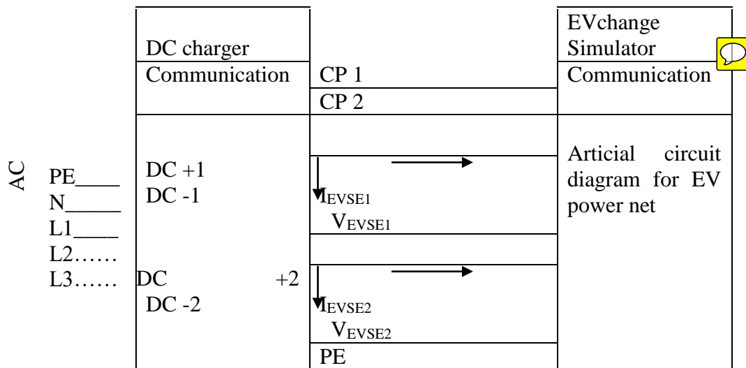
FIG. 31 STANDARD TEST SETUP CIRCUIT DIAGRAM
