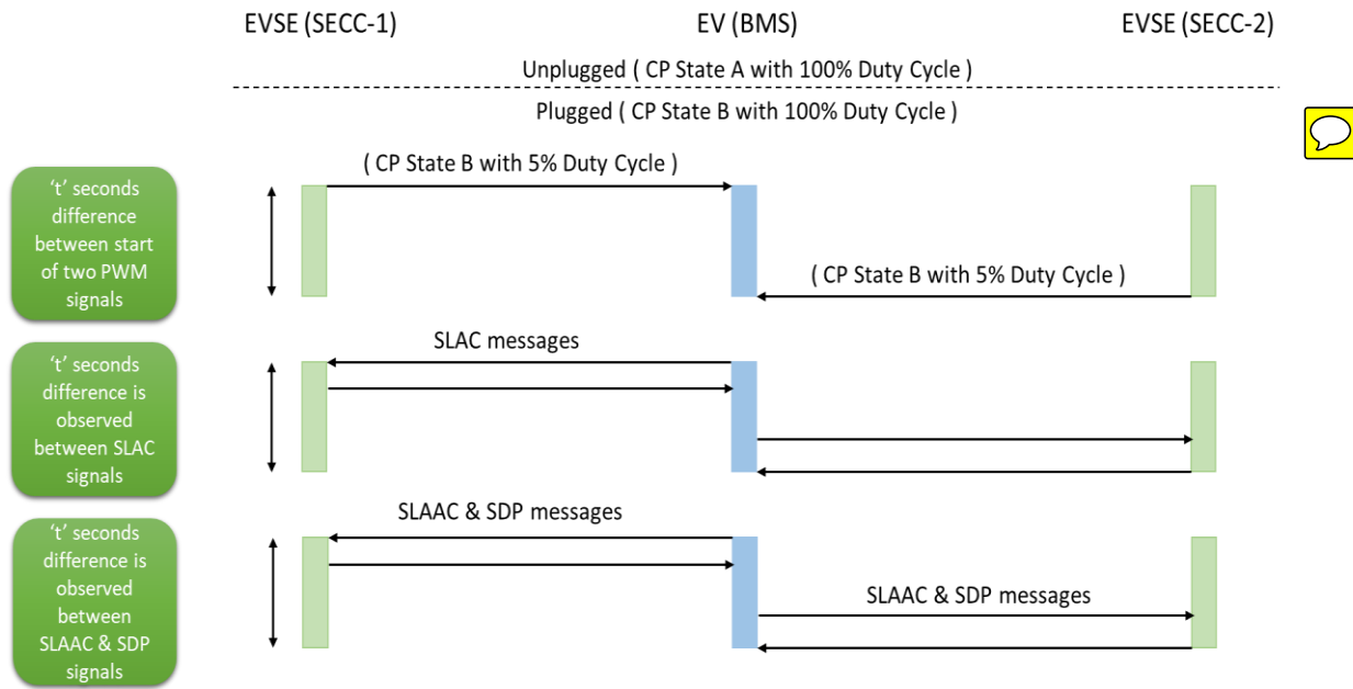
FIG. 45 CHARGING PHASES FOR DUAL GUN CHARGING
