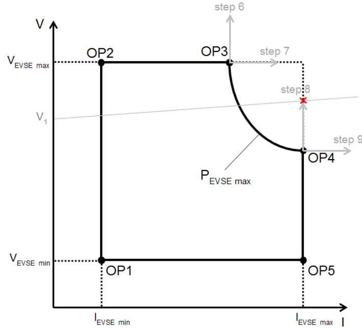
FIG. 32 TEST POINT GRID
