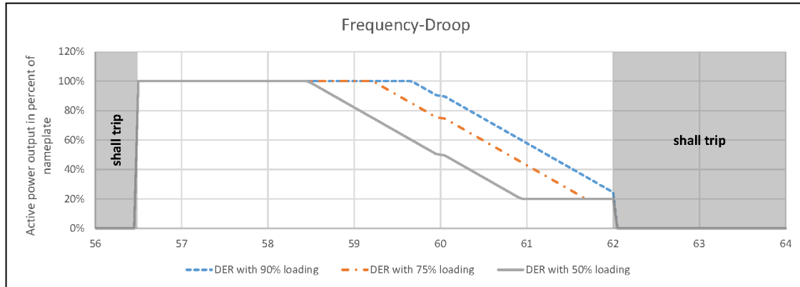
Figure H.11—Example of a three frequency-droop function curves with a 5% droop, 36 mHz deadband, and 20% minimum active power output for DER operating at different pre-disturbance levels of nameplate rating (50%, 75%, and 90%)
