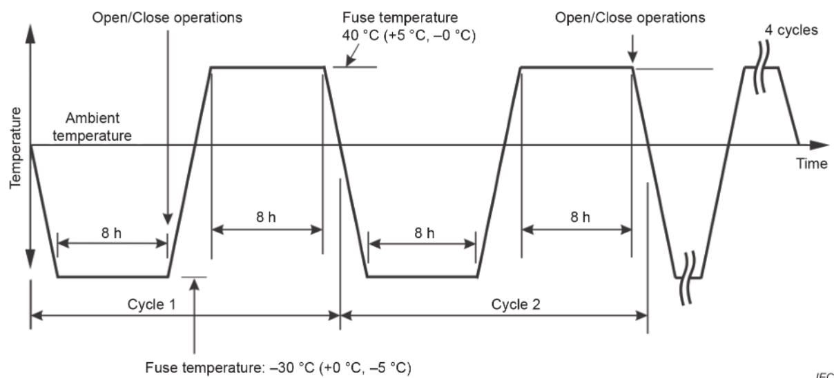
Figure 1 – Test sequence
