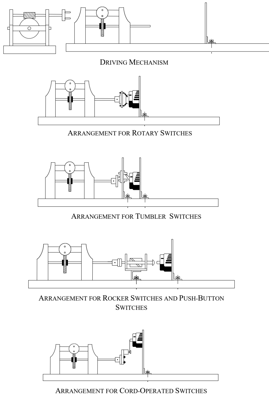
FIG. 101 EXAMPLE OF APPARATUS FOR TESTING THE MAKING AND BREAKING CAPACITY AND THE NORMAL OPERATION OF SWITCHES IN SWITCHED SOCKET-OUTLETS
