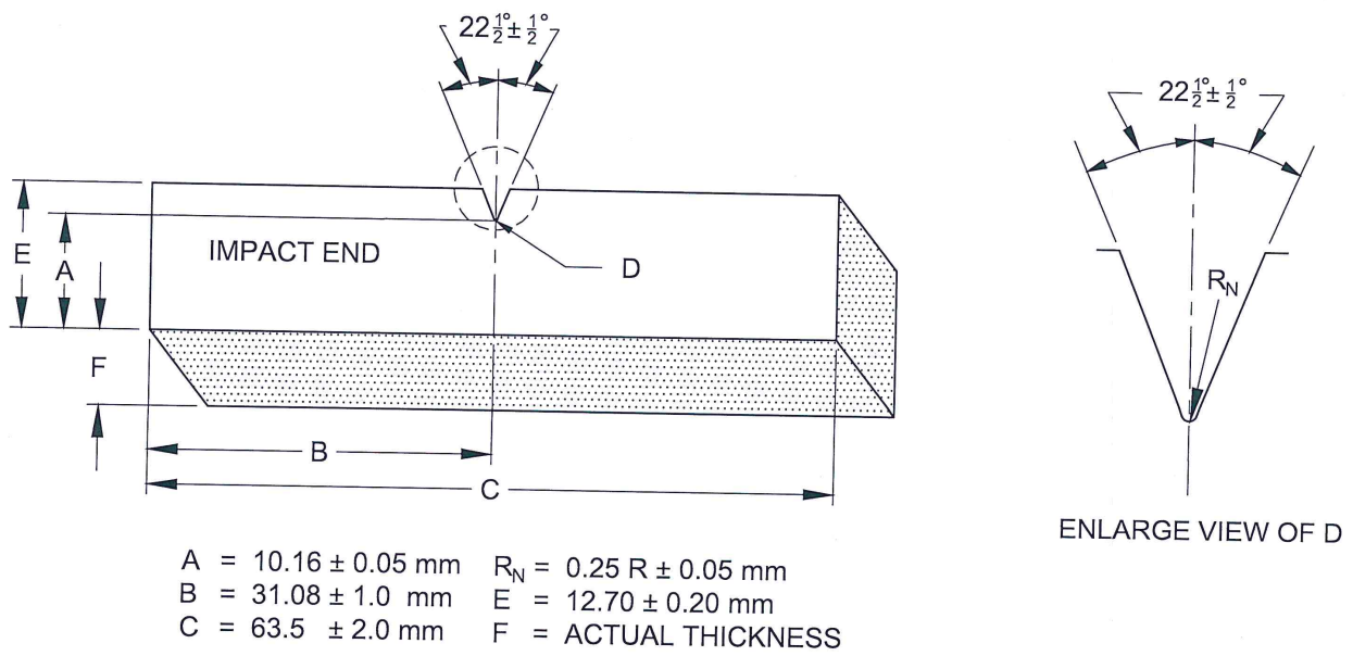
FIG.4 DIMENSIONS OF IZOD IMPACT TEST SPECIMEN
