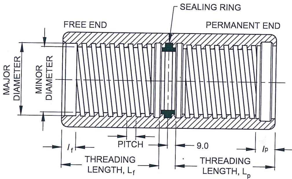
1D THREADS PROFILE OF COLUMN PIPE
