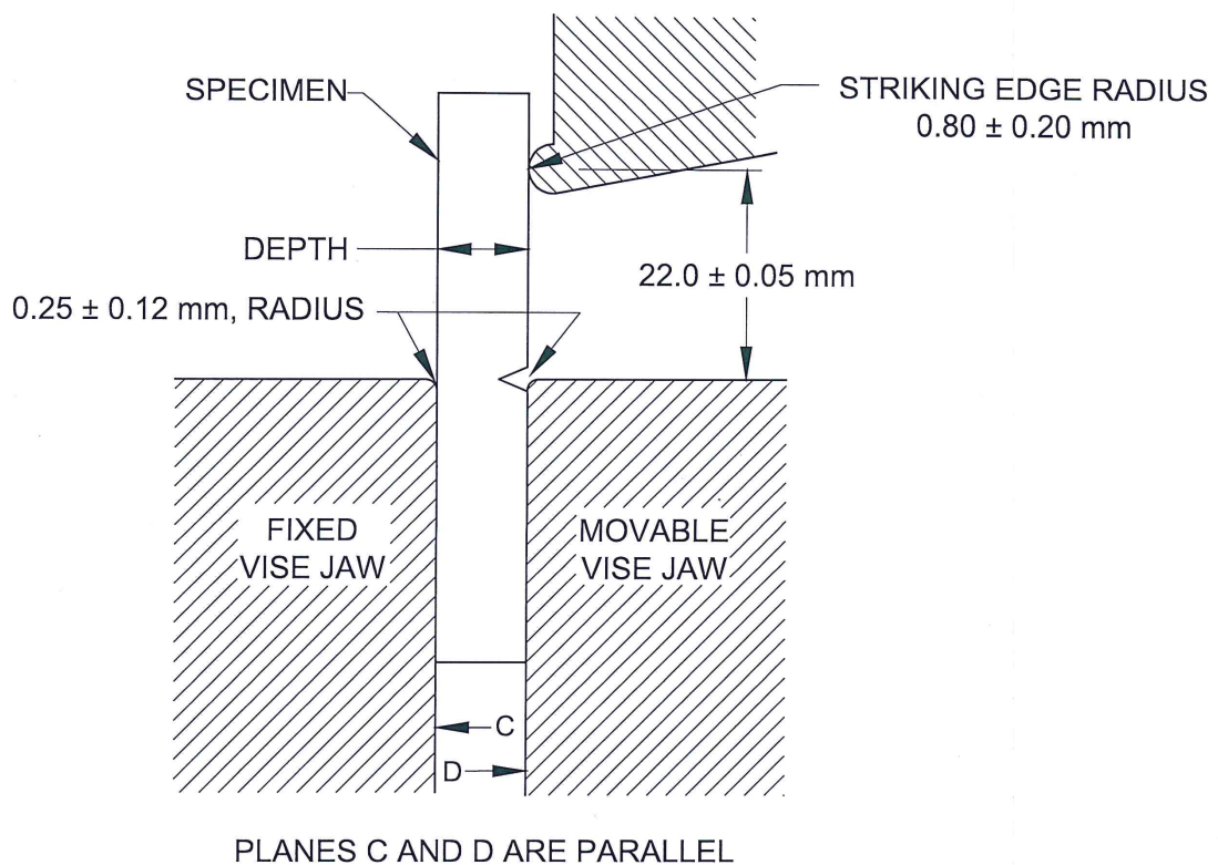
FIG. 5 RELATIONSHIP OF VISE, SPECIMEN AND STRIKING EDGE
