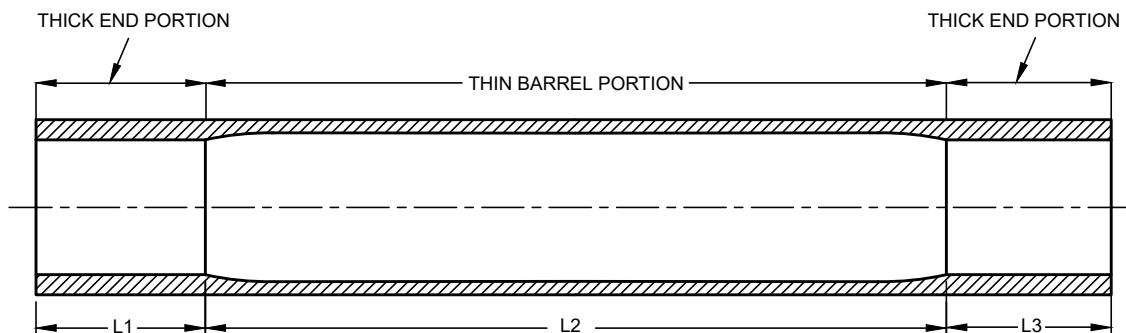
1A UNTHREADED PIPE
