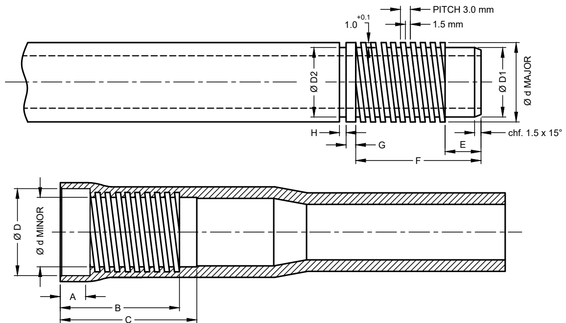
FIG. 2 BELL ENDED COLUMN PIPES WITH INTERNAL THREADS AT ONE END AND SPIGOT AT ANOTHER END WITH EXTERNAL THREADS
