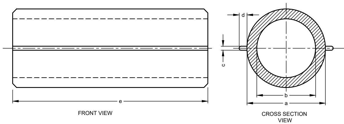
1C RIBBED COUPLER BEFORE THREADING
