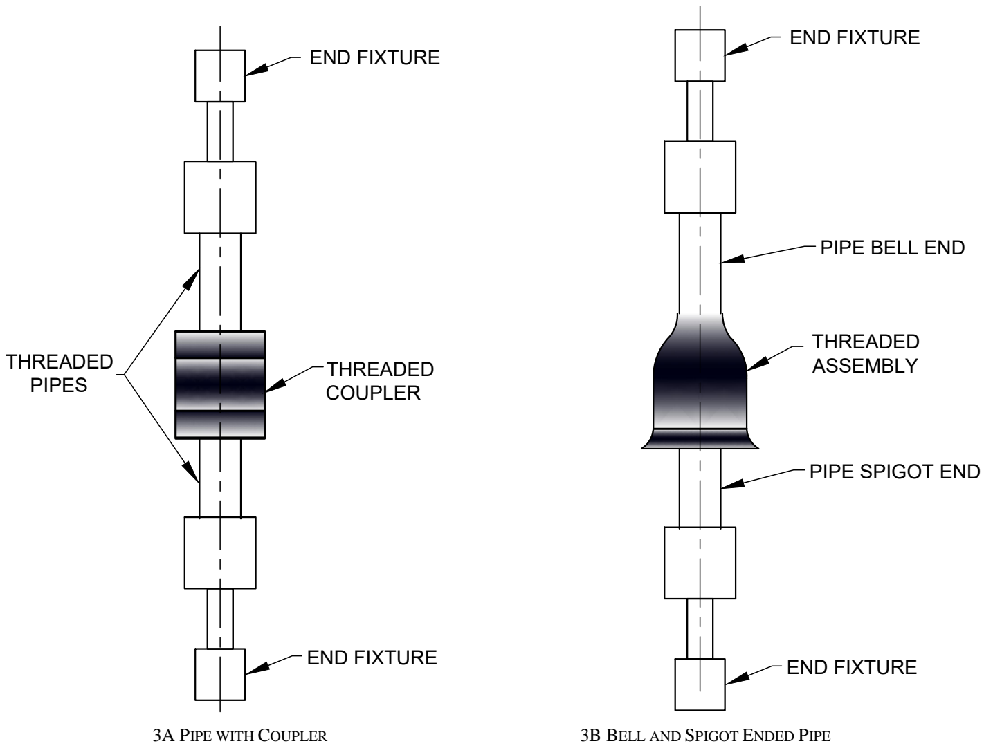
FIG. 3 TYPICAL ULTIMATE BREAKING LOAD ASSEMBLY
