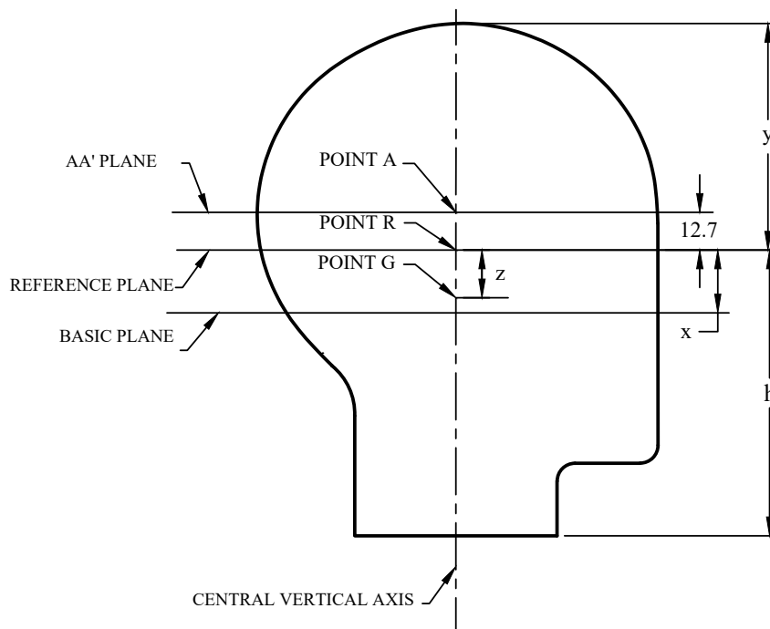
SECTION ON VERTICAL LONGITUDINAL PLANE
