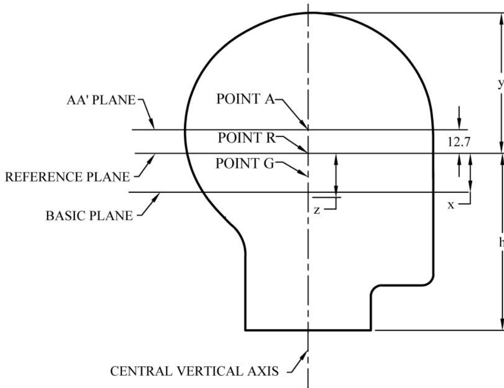
SECTION ON VERTICAL LONGITUDINAL PLANE
