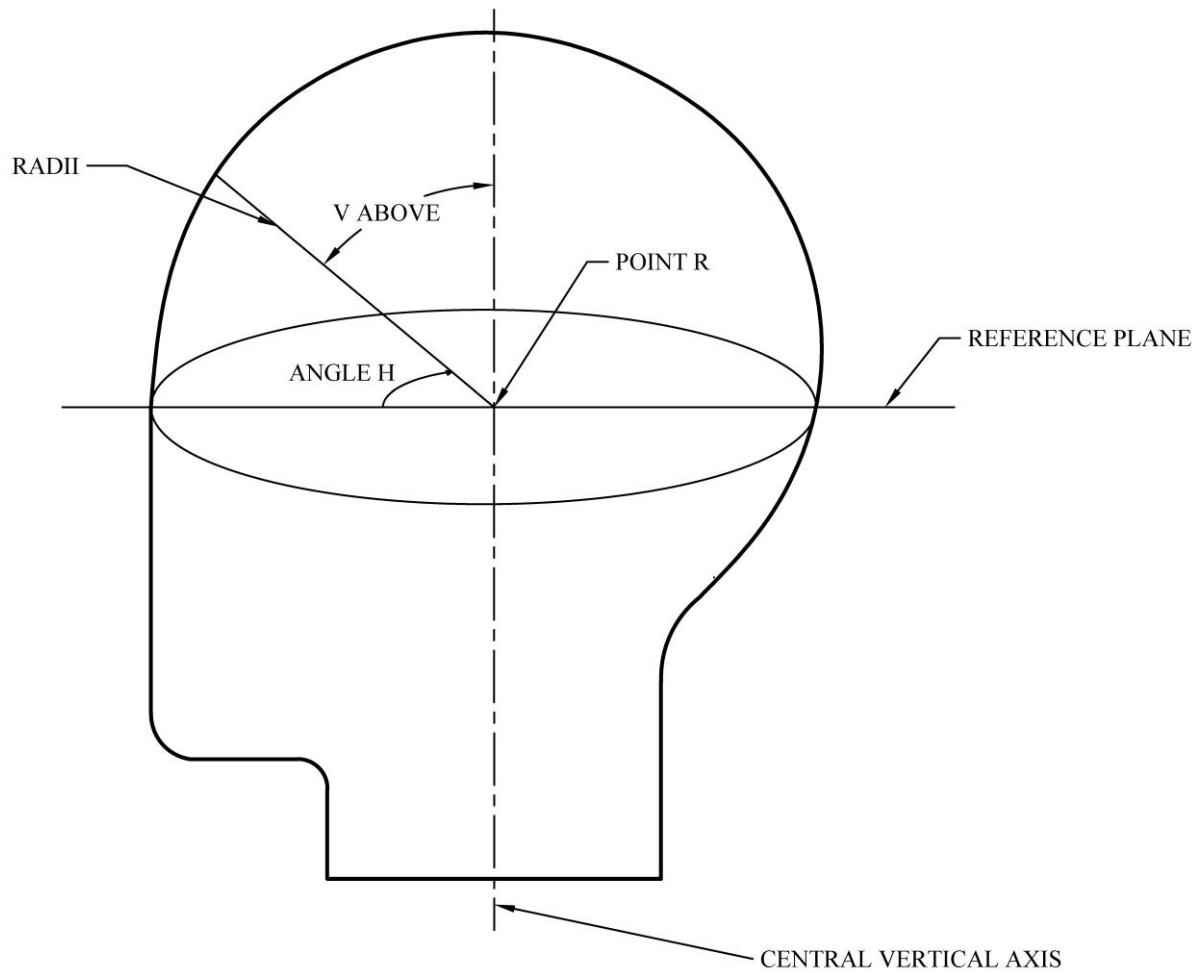
FIG. 2 RADII, ANGLE H, AND ANGLE V OF A HEADFORM
