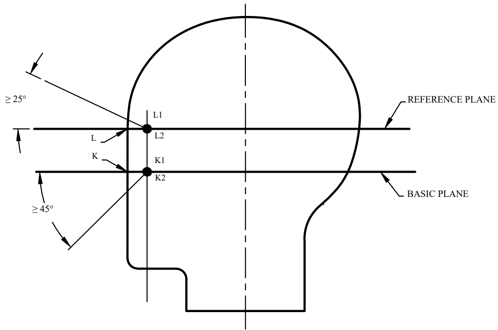
1A SECTION OF HEADFORM IN LONGITUDINAL VERTICAL PLANE
