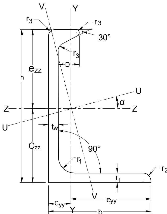
FIG. 1 HOT ROLLED STEEL BULB ANGLE
