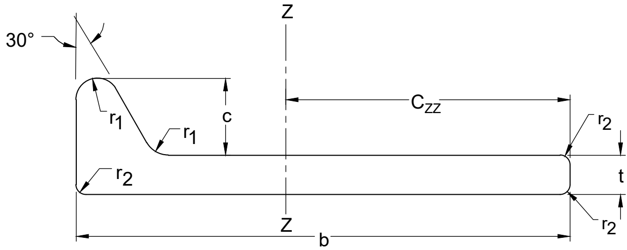
FIG. 2 TYPICAL BULB FLAT
