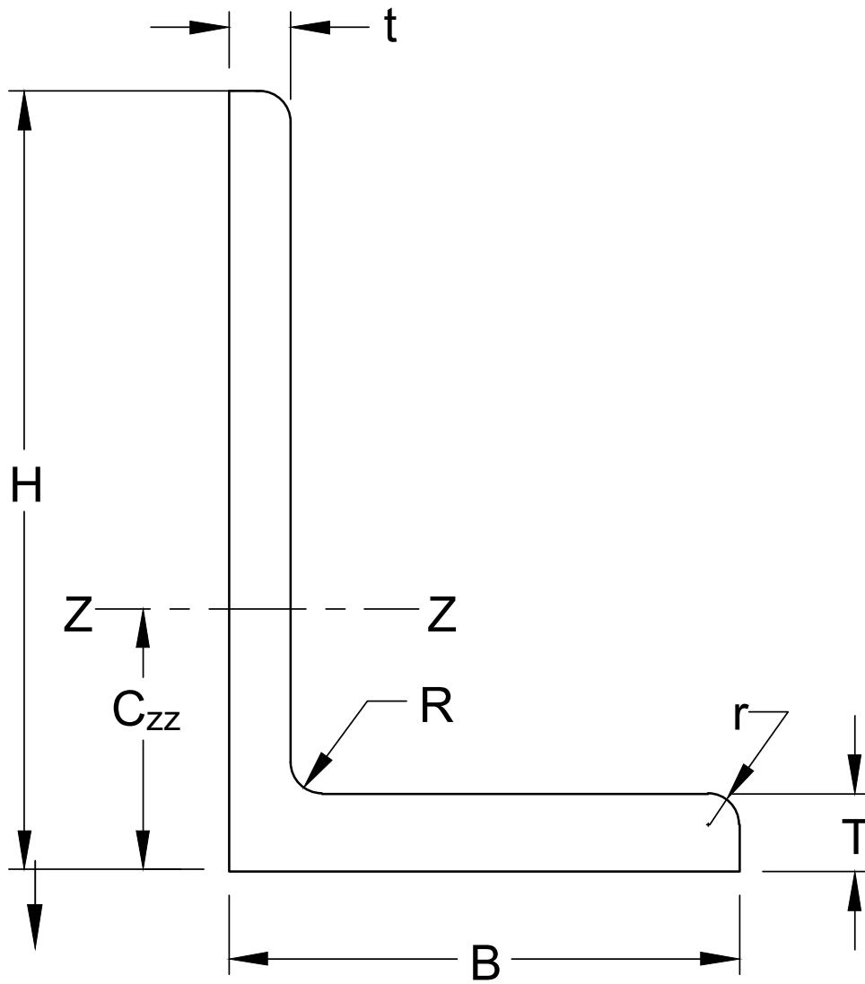
FIG. 3 TYPICAL 'L' SECTION
