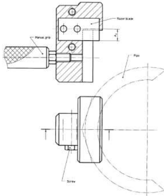
Fig. 4 Notching Device
