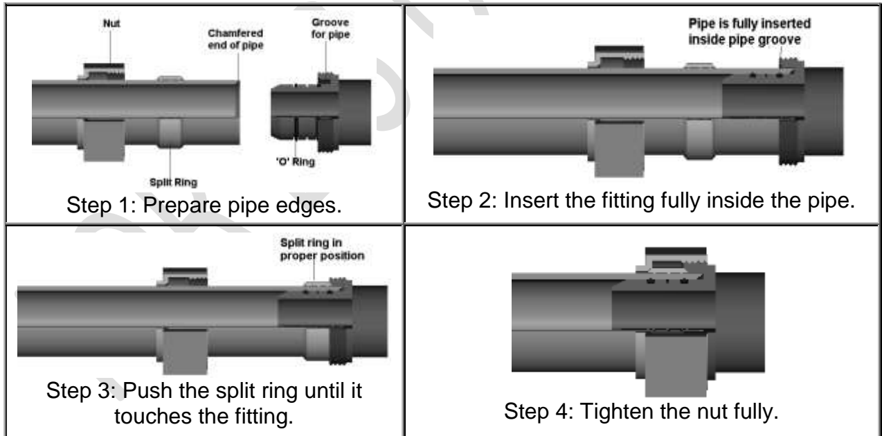
Fig. 13 Jointing using Brass Internal Sealing Fittings
