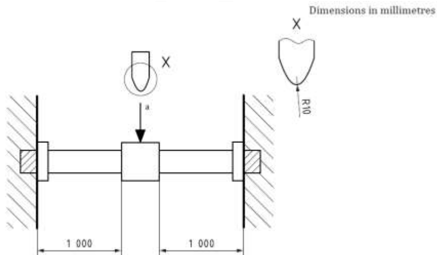
Fig. 9 Impact resistance test assembly
