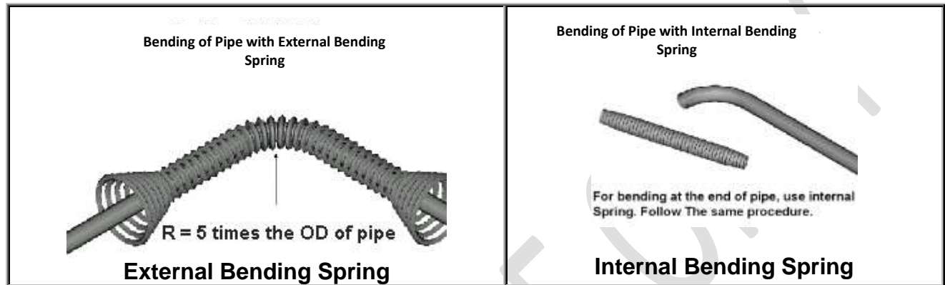
Fig. 14 Bending Spring
