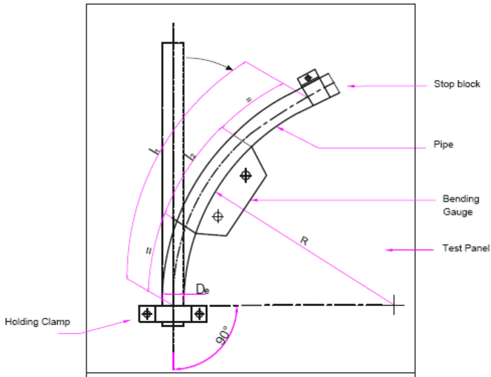
Fig. 6 Diagram of Typical Bending Apparatus
