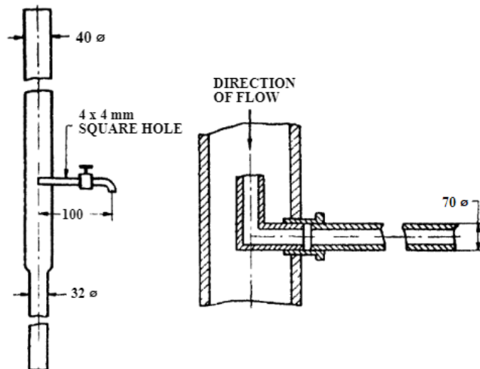
FIG. 10 CONTINUOUS SAMPLER
