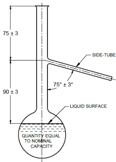
FIG. 1 DISTILLATION FLASKS
