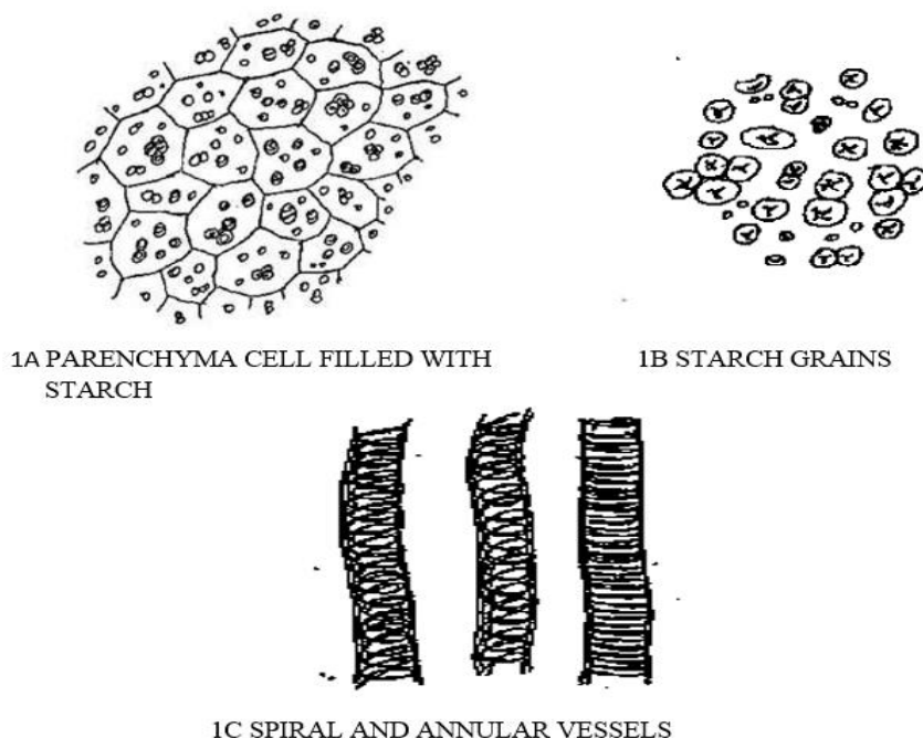
FIG. 1: SURANJAN POWDER MICROSCOPY
