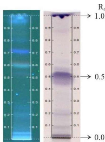
UV 366 nm After derivatization
