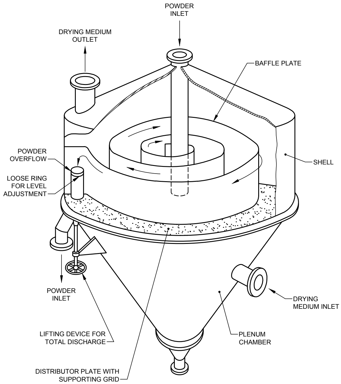
FIG. 1 NOMENCLATURE OF FLUID BED DRYER
