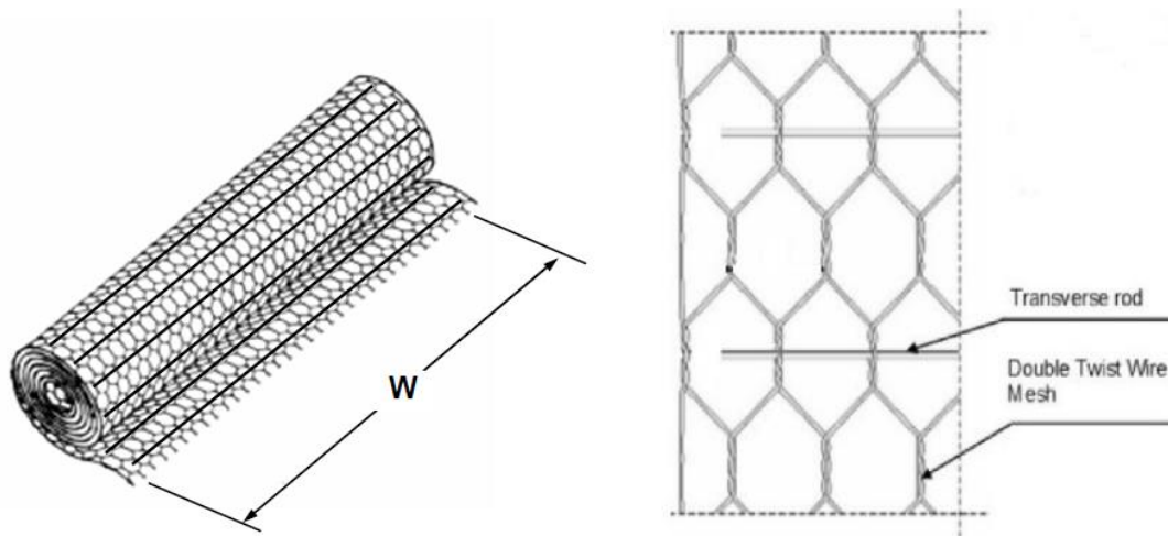
FIG. 12 PAVEMENT REINFORCEMENT MESH
