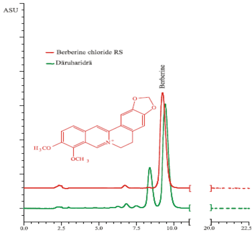
FIG. 3 HPLC CHROMATOGRAM OF DARUHARIDRA ( Berberis aristata DC) STEM WITH BERBERINE CHLORIDE AS RS
