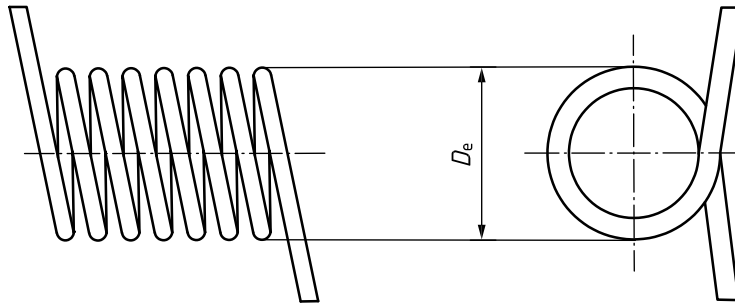
Figure 6 — Outside diameter ( D_e )
