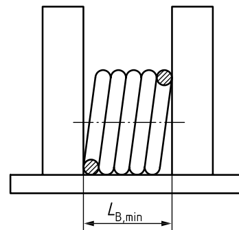
d) Tolerance lower limit check with gauge ( L_B \geq L_{B,min} ) (GO/out of tolerance)
