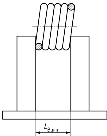
c) Tolerance lower limit check with gauge ( L_B < L_{B,min} ) (NO GO/within tolerance)
