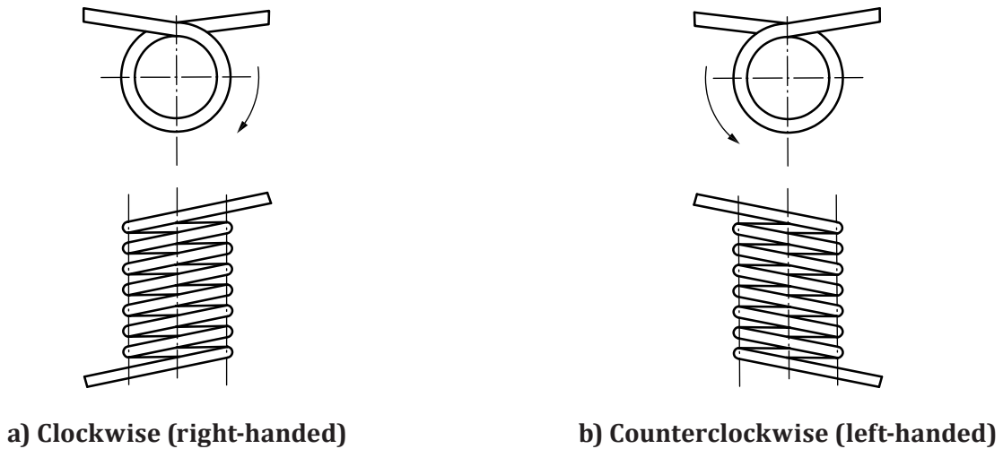
Figure 16 — Coil direction
