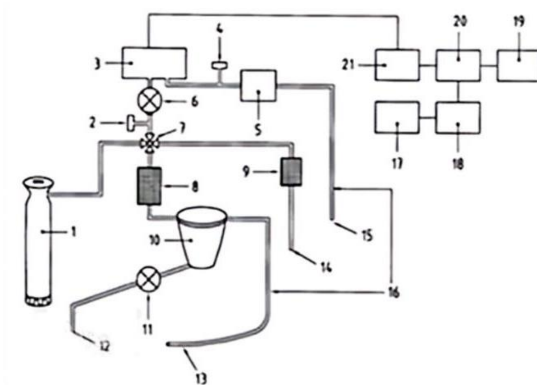
FIG. 1 DIAGRAMMATIC ILLUSTRATION OF AN INSTRUMENT FOR MEASURING VEHICLE EXHAUST EMISSIONS
