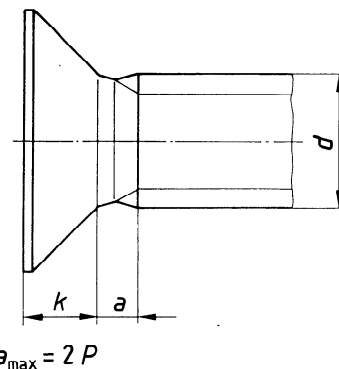
Figure 2 — Screw without underhead shoulder
