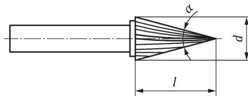
Figure 1 — Hardmetal burr, style M
