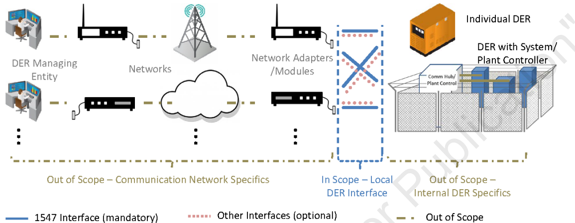
Figure 4 —Control protocol in/out of scope mapping
