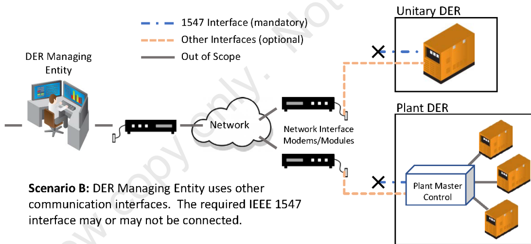
Figure D.2—DER using custom interface
