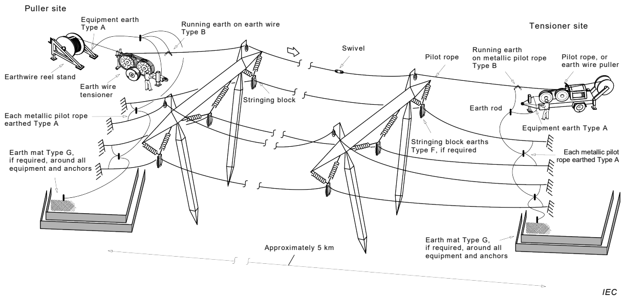
f) Transmission – Installing the earth wire
