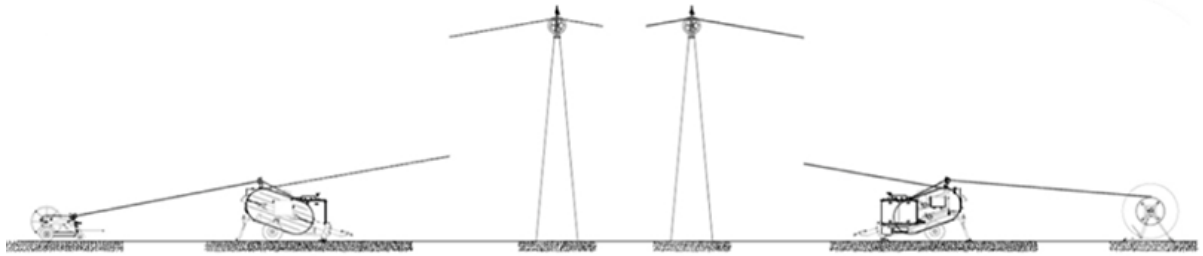
j) Transmission – n \times n stringing method
