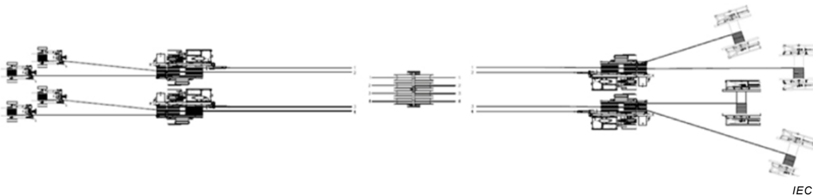
k) Transmission – n \times n reconductoring stringing method
