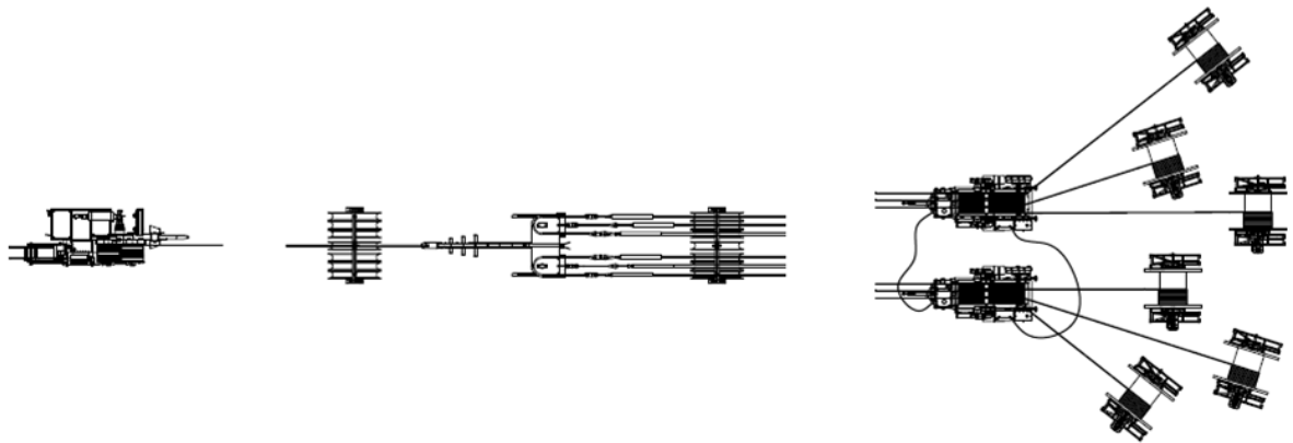
i) Transmission – 1 × n stringing method
