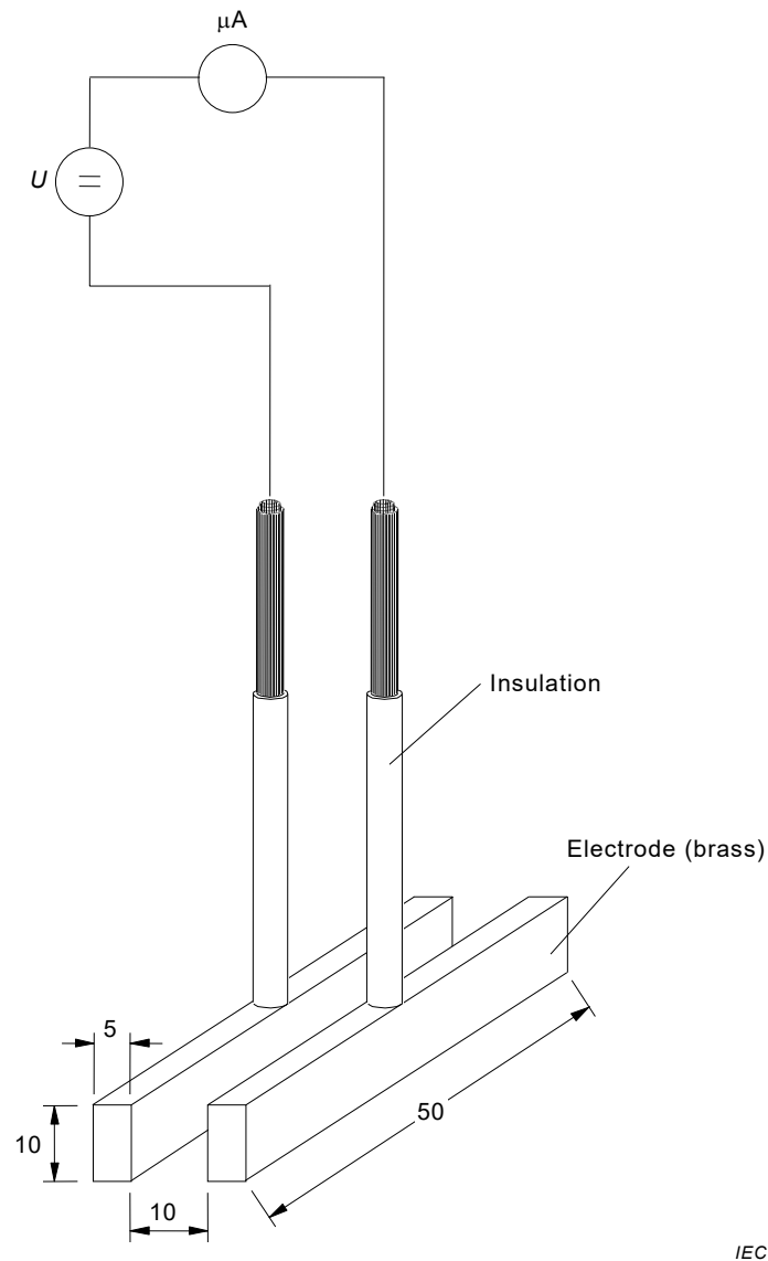
Figure 2 – Test arrangement for the insulation resistance test of the filling material
