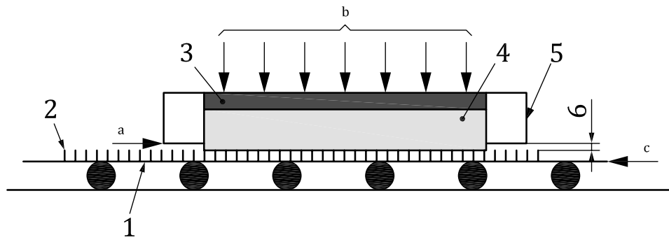
a) Constant area direct shear test (typical layout) for sand/generic soil — Geosynthetic interface
