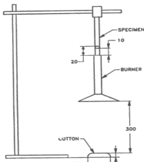
FIG. 1 VERTICAL BURNING-BEHAVIOUR TEST APPARATUS
