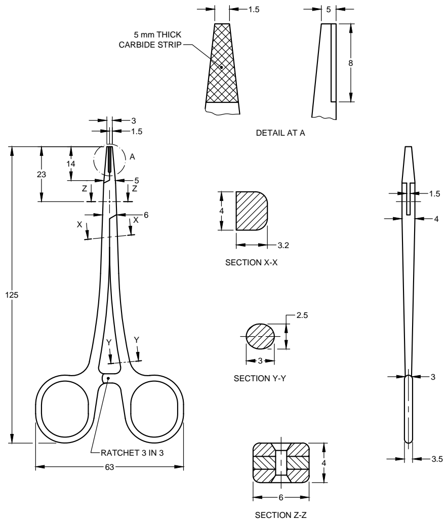
FIG. 1 NEEDLE HOLDER
