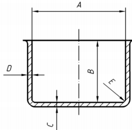
FIG. A-1 CHARACTERISTICS OF TEST VESSELS
