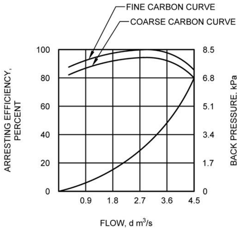
FIG. 2 PERFORMANCE OF SPARK ARRESTER UNDER LABORATORY TEST WITH AIR
