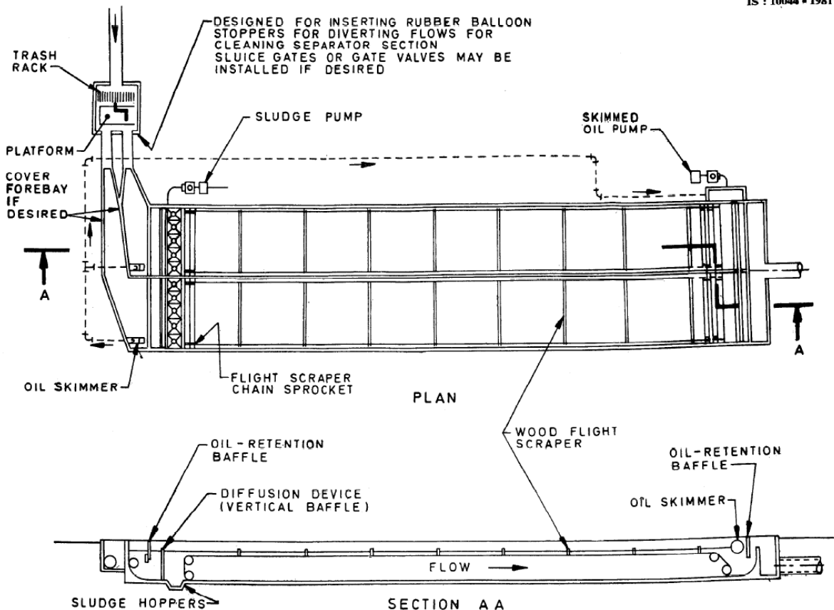
FIG. 1 API OIL-WATER SEPARATOR
