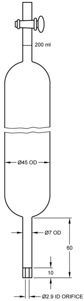
All dimensions in millimetres. FIG. 1 FOAM PIPETTE
