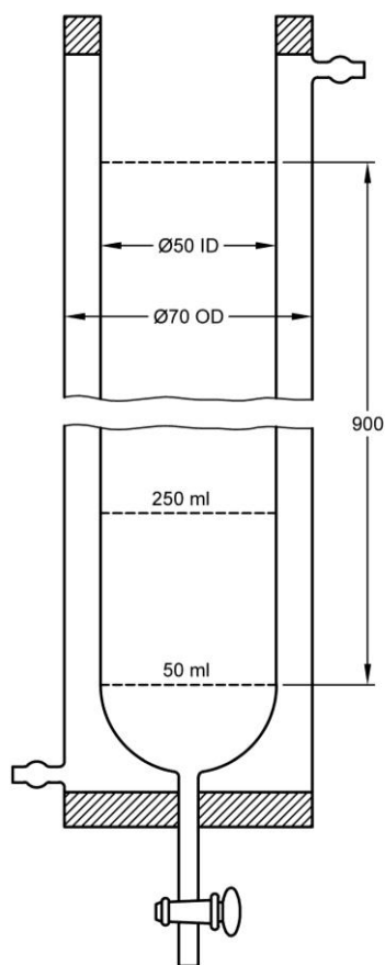
All dimensions in millimetres. FIG. 2 FOAM RECIEVER
