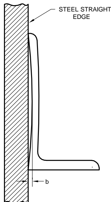
FIG. 8 MEASUREMENT OF DEVIATION IN FLATNESS OF WEB
