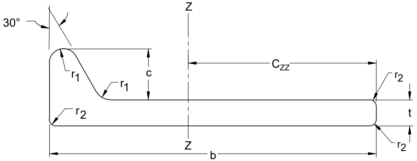
FIG. 2 TYPICAL BULB FLAT
