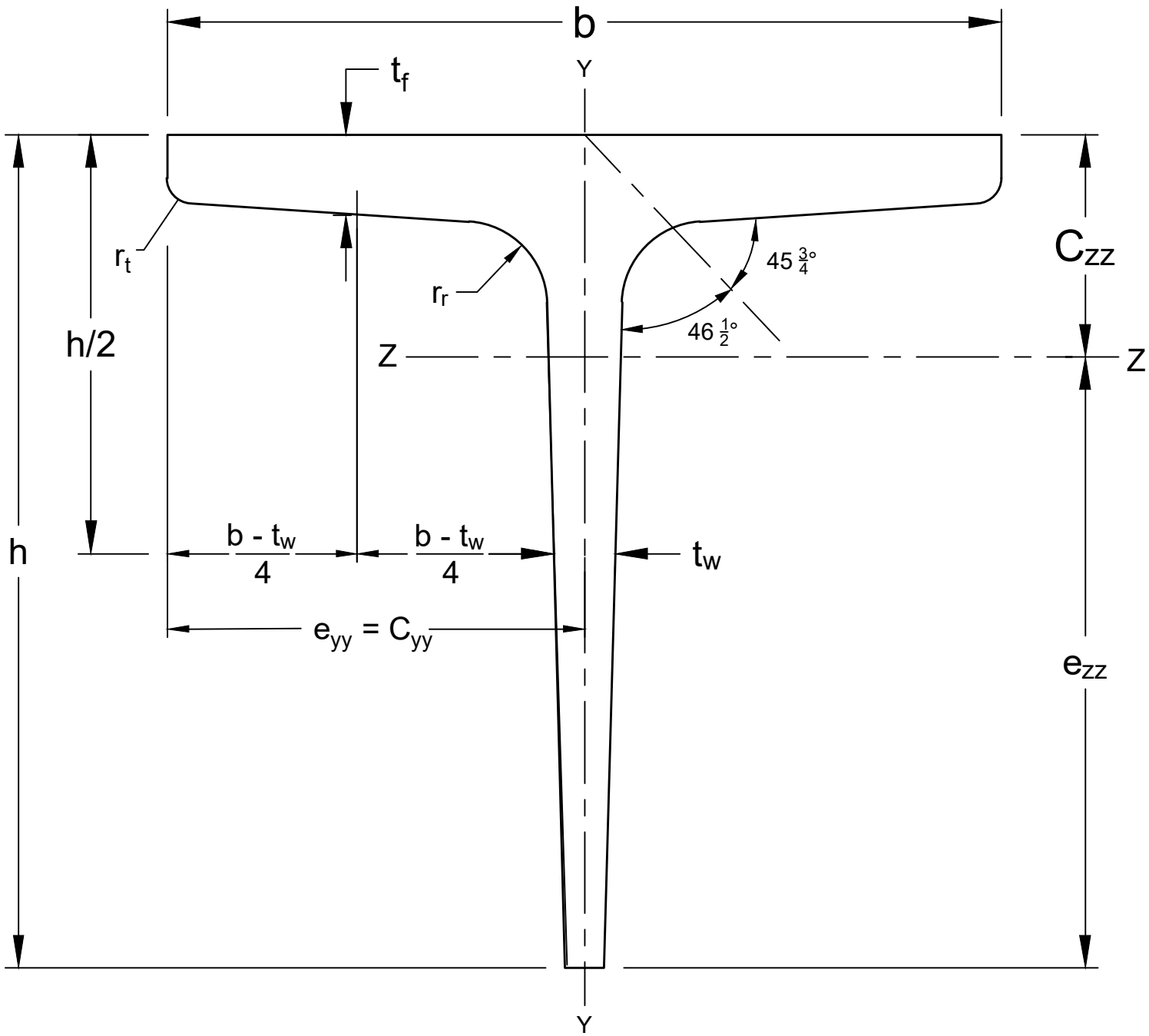
FIG. 1 ROLLER NORMAL TEE BAR (ISNT)
