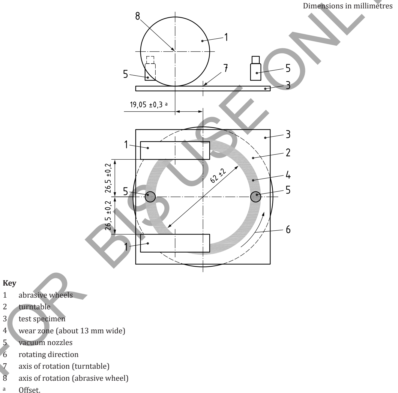
Figure 2 — Schematic diagram of the turntable abrasion tester
