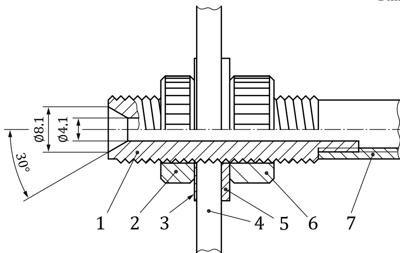
Figure 4 — Example of disc probe
