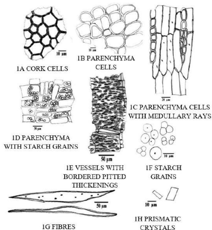
FIG. 1 POWDER CHARACTERS OF AGNIMANTHA ( Clerodendrum phlomidis L. f.) ROOT
