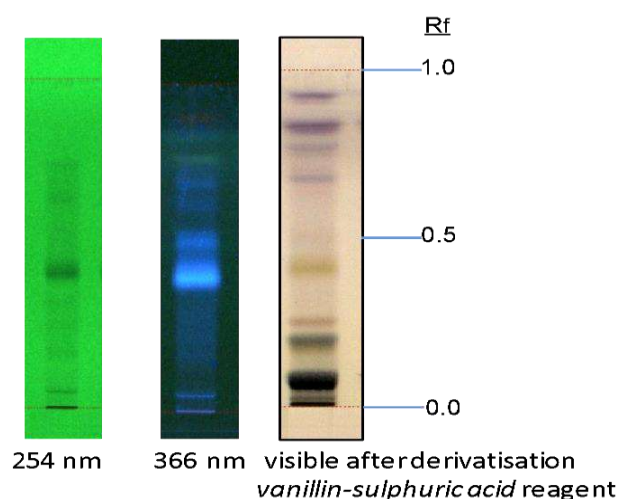
FIG. 2 TLC FINGERPRINTS OF AGNIMANTHA ( Clerodendrum phlomidis L.f.) ROOT
