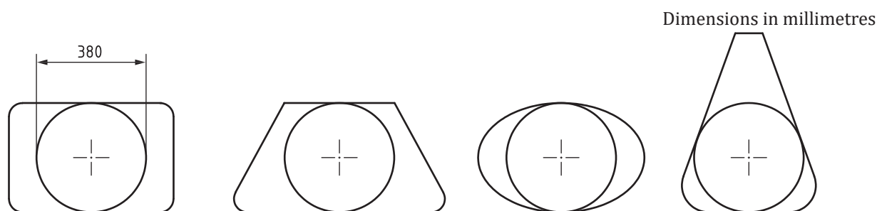
Figure 2 — Measurement of minimum clear opening
