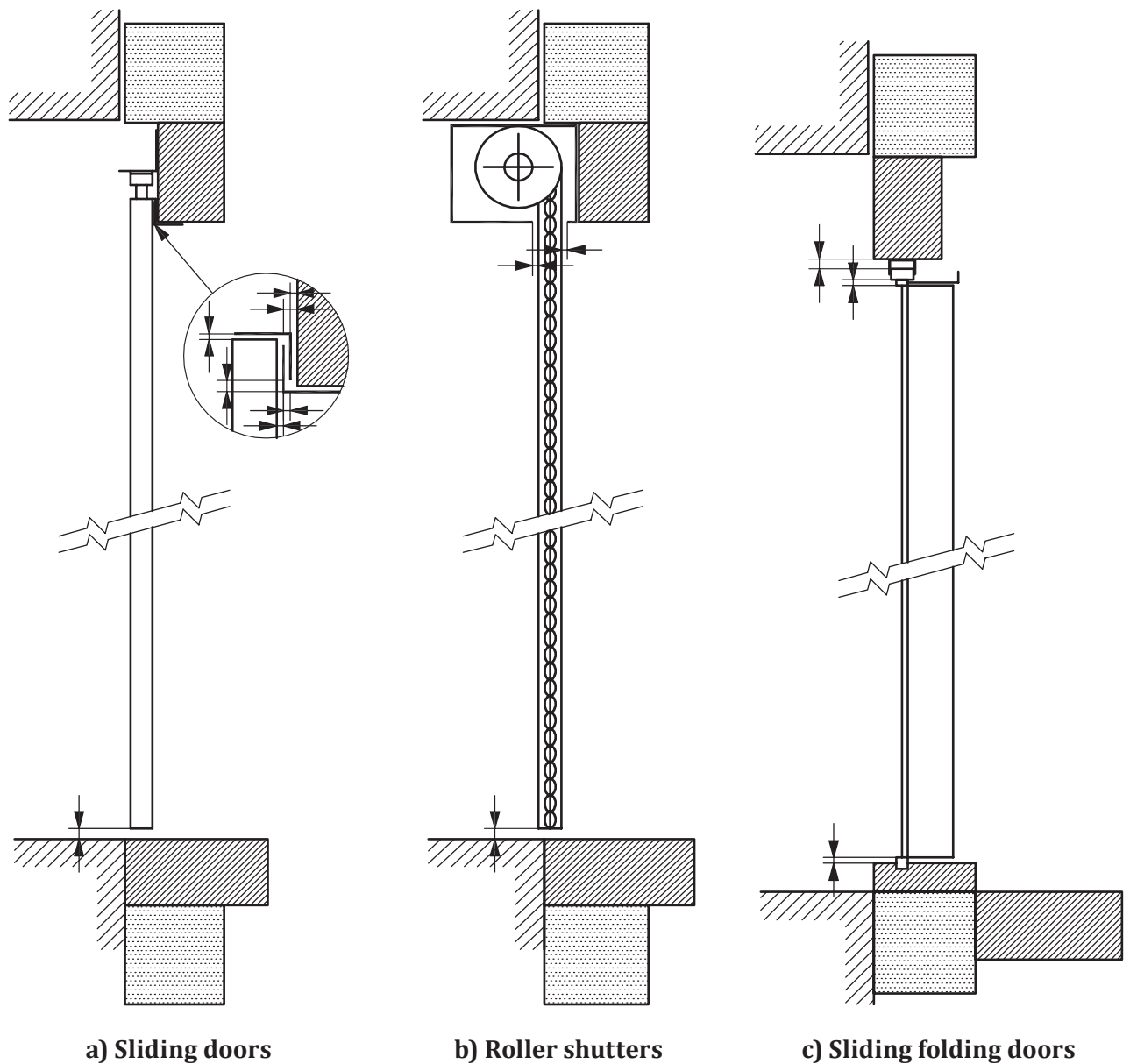
Figure 12 — Examples of gap measurements — Vertical sections
