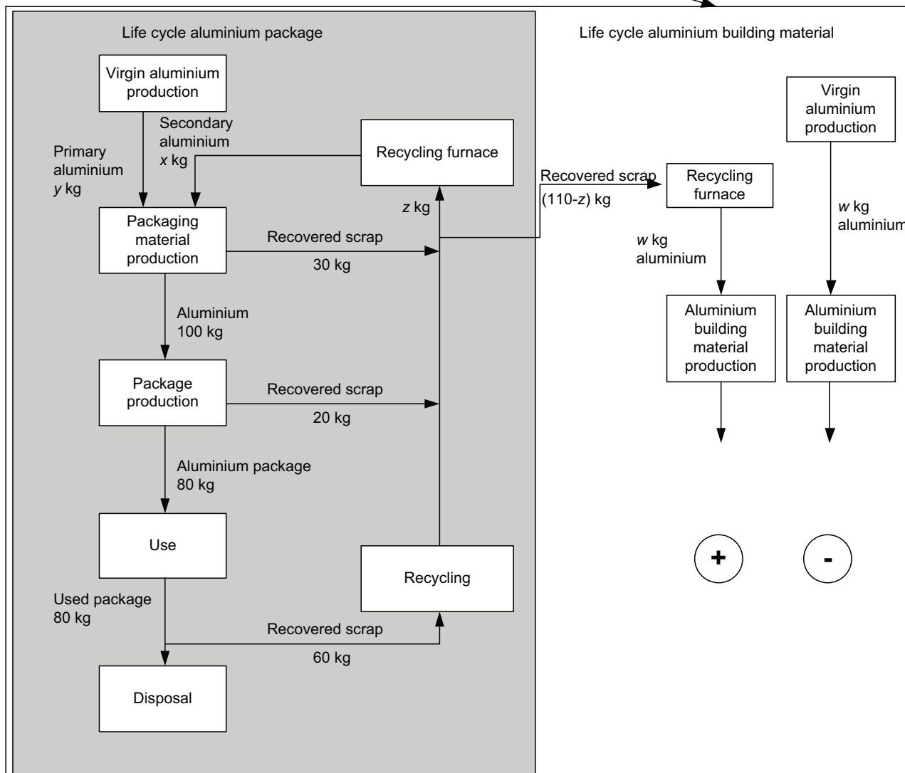
Figure 16 — Open-loop with closed-loop recycling procedure for aluminium package with expanded system boundaries (example for other product life cycles: aluminium building material)
